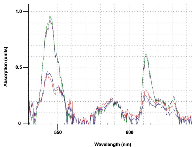
Figure 3. Absorption spectra of the reaction solution for the synthesis of 9 : 0 min (red), 3 min (blue), 5 min (violet) and 10 min (green).
