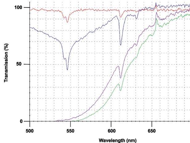
Figure 2. Transmission spectra of the reaction solution for the synthesis of 6 : 0 min (red), 10 min (blue), 20 min (violet) and 30 min (green).
