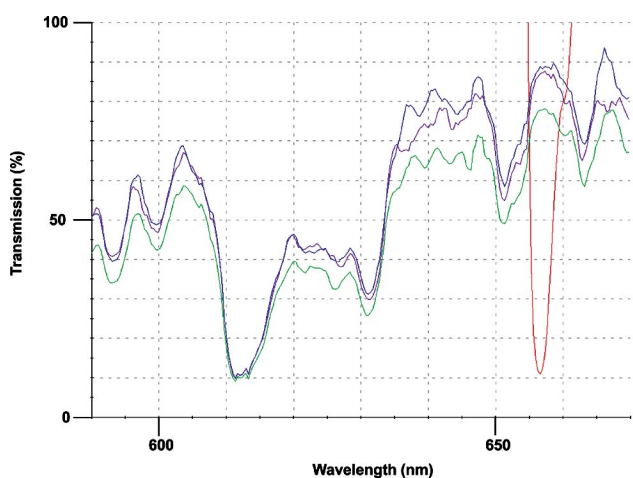
Figure 1. Transmission spectra of the reaction solution for the synthesis of 3 : 0 min (red), 3 min (blue), 10 min (violet) and 15 min (green).
