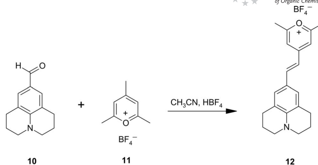
Scheme 3. Synthesis of 12 .
