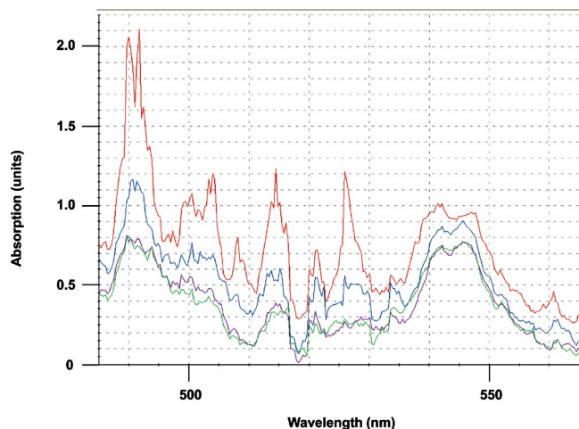
Figure 5. Absorption spectra for the reaction solution for the synthesis of 14 : 0 min (red), 3 min (blue), 5 min (violet) and 8 min (green).
