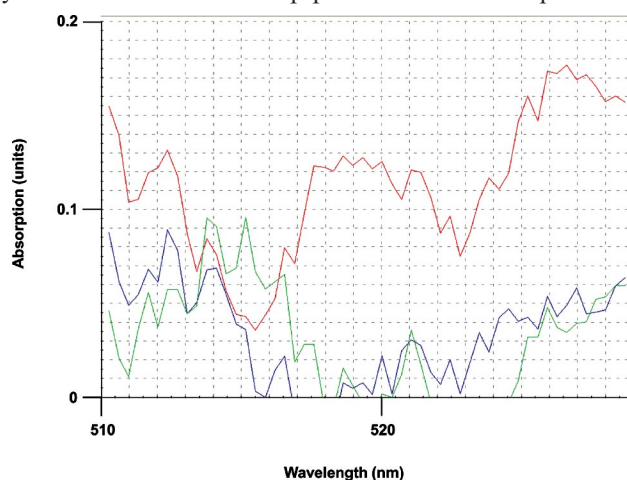
Figure 4. Absorption spectra of the reaction solution for the synthesis of 12 : 0 min (red), 3 min (blue) and 5 min (green).
