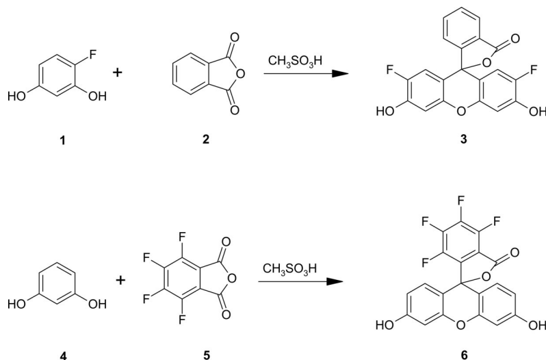
Scheme 1. Syntheses of the fluorinated dyes 3 and 6 .
